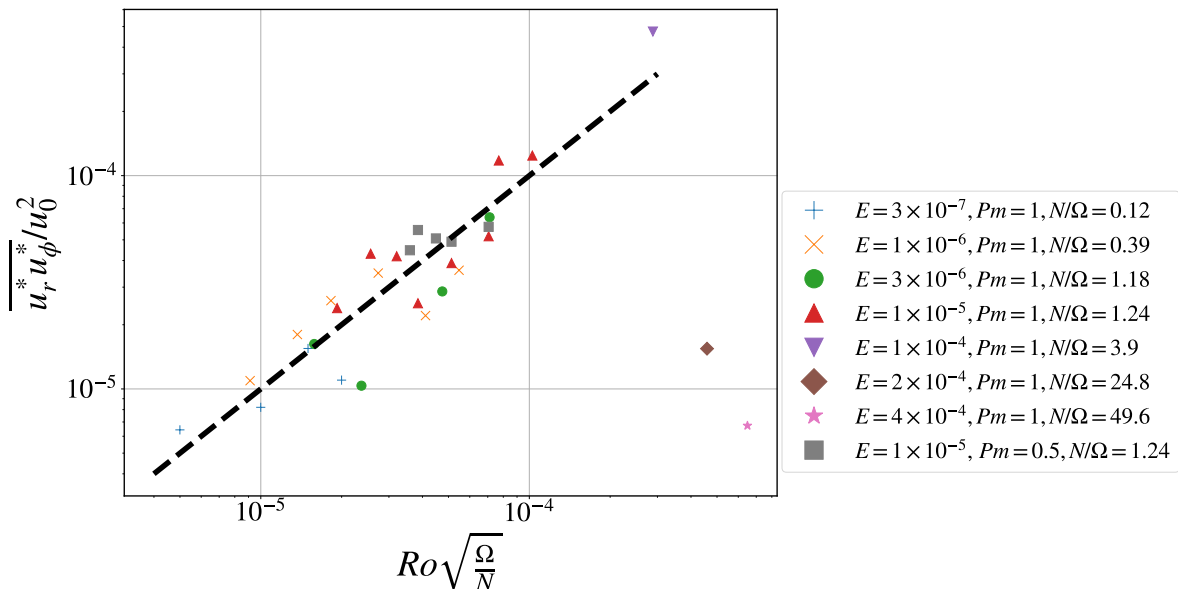
FIG. 5. Scaling law for the dimensionless Reynolds stress \overline{u_r^* u_\phi^*} / u_0^2 . This Reynolds stress is measured in the dynamo region, for \pi/4 < \theta < 3\pi/4 and 0.45 < r/r_0 < 0.55 . Here we show simulations only for Pm \leq 1 , as they correspond to simulations with the highest Reynolds number, relevant for astrophysical applications (see discussion).
