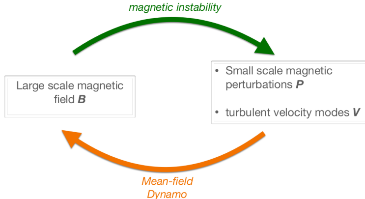
FIG. 6. Diagram illustrating the mechanism described by the model in Eqs. (9)-(11): a large-scale magnetic field B is destabilized through some linear MHD instability, generating small-scale perturbations. At large Rm, Re , these perturbations are chaotic and drive turbulent velocity fluctuations, which then regenerate the initial large-scale field through a mean-field dynamo.
