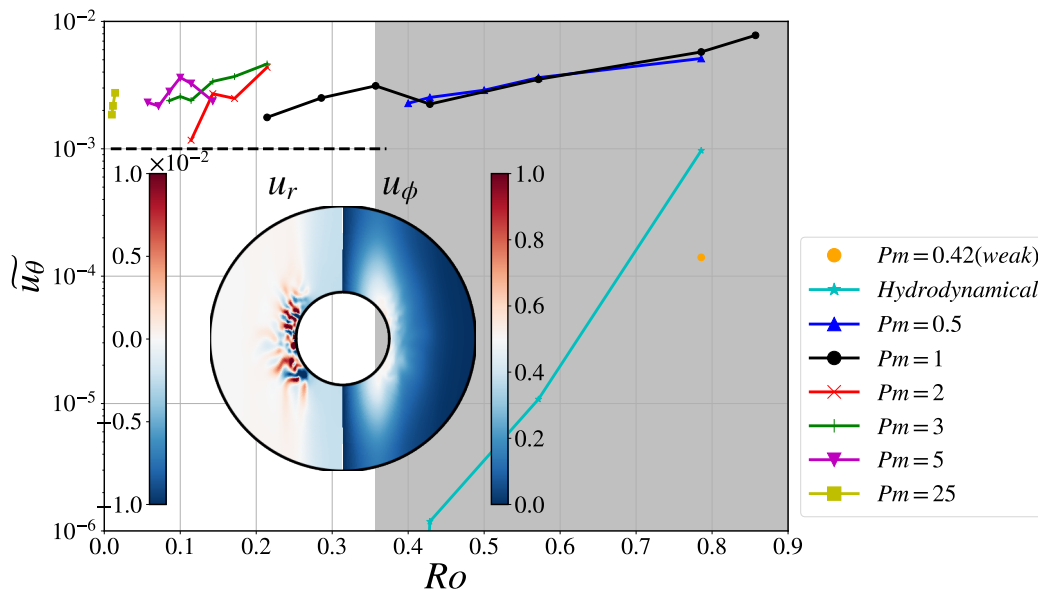
FIG. 2. Bifurcation of the velocity perturbations as a function of the Rossby number for Ek = 10^{-5} and N/\Omega = 1.24 . For each run, \tilde{u}_\theta = \sqrt{\langle (u_\theta - \bar{u}_\theta)^2 \rangle_t} is measured locally in the equatorial plane where the dynamo is the strongest, at r = 0.55r_o . Inset: Snapshot of the velocity field for the run Ro = 0.14 , Pm = 2 at \phi = 0 .
