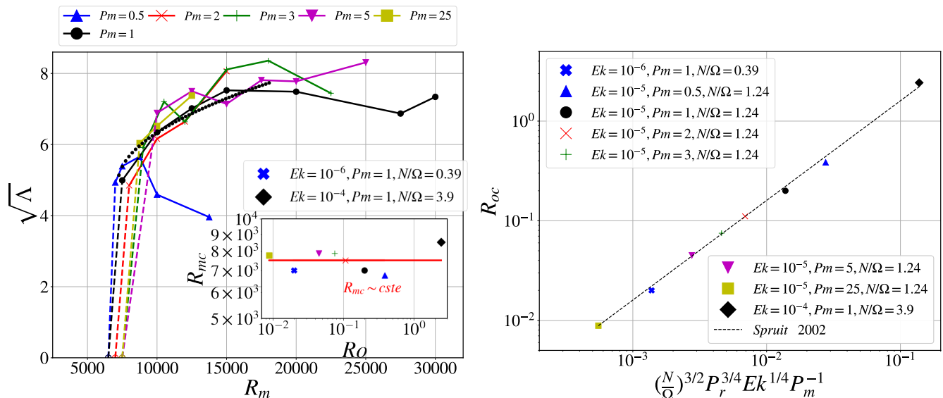
FIG. 4. Left: \sqrt{\Lambda} as a function of Rm for different Pm . The normal form of the bifurcation is relatively well fitted by the nonlinear model (dotted line) developed in Sec. IV. Inset: The critical magnetic Reynolds number of the dynamo, computed for each Pm , is independent of the kinetic Reynolds number. Right: Critical Rossby number for the dynamo, compared to Spruit's prediction [28] (dashed line).
