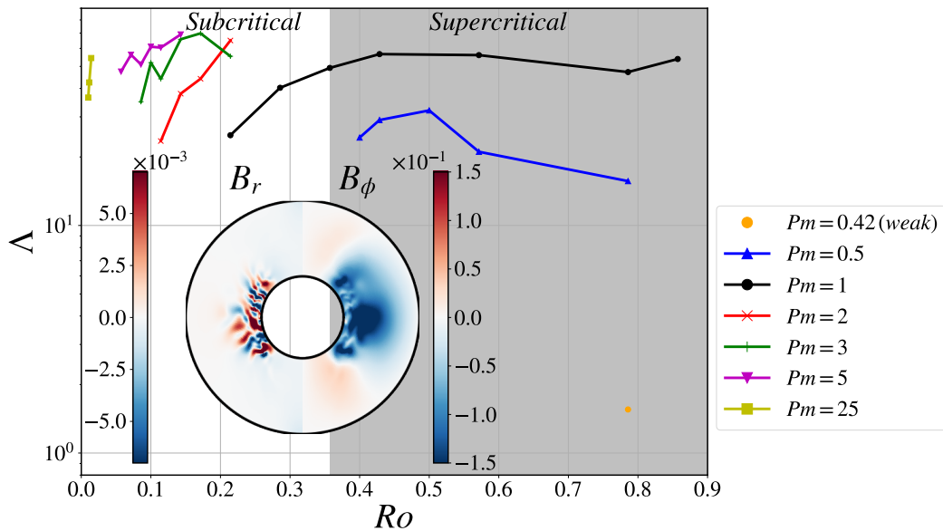
FIG. 1. Bifurcation diagram of Elsasser number vs Rossby number for Ek = 10^{-5} and N/\Omega = 1.24 . Taking advantage of the subcritical nature of the bifurcation, the dynamos at Ro < Ro_h have been obtained either by restarting from the solution obtained at Pm = 1 , or initialized with a dipolar magnetic field strong enough to reach the basin of attraction of the corresponding solution (see text for details). Inset: Snapshot of the magnetic field components B_r and B_\phi for the run Ro = 0.14 , Pm = 2 at \phi = 0 .
