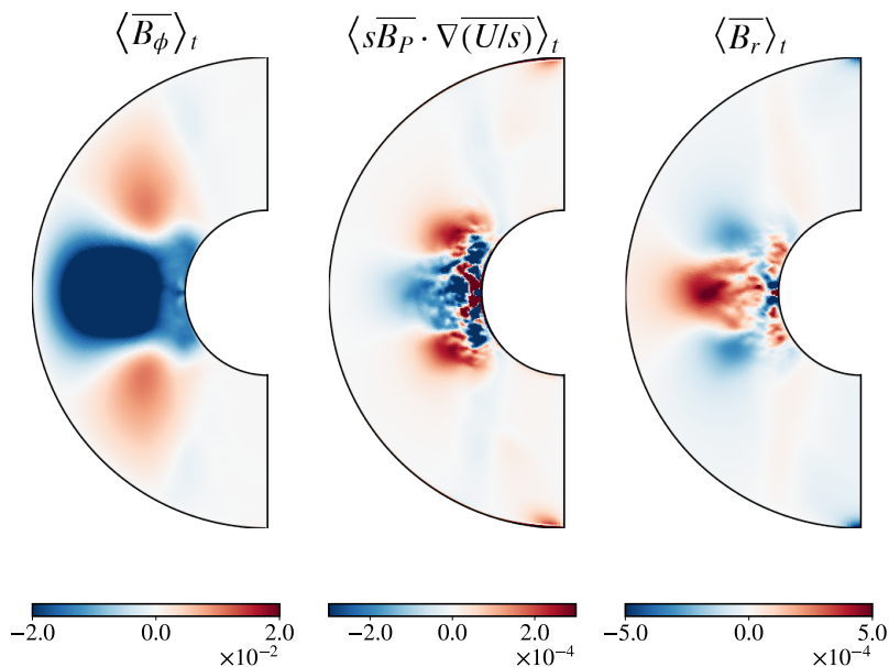
FIG. 7. From left to right: (a) map of \overline{B_\phi} , averaged in time and in the azimuthal direction. (b) Same, for the \omega -effect, \overline{B_P} \cdot \nabla \overline{U} . (c) Same for \overline{B_r} . All the maps are computed on the saturated phase for R_o = 0.78 , Pm = 1 , Ek = 10^{-5} , N/\Omega = 1.24 .
