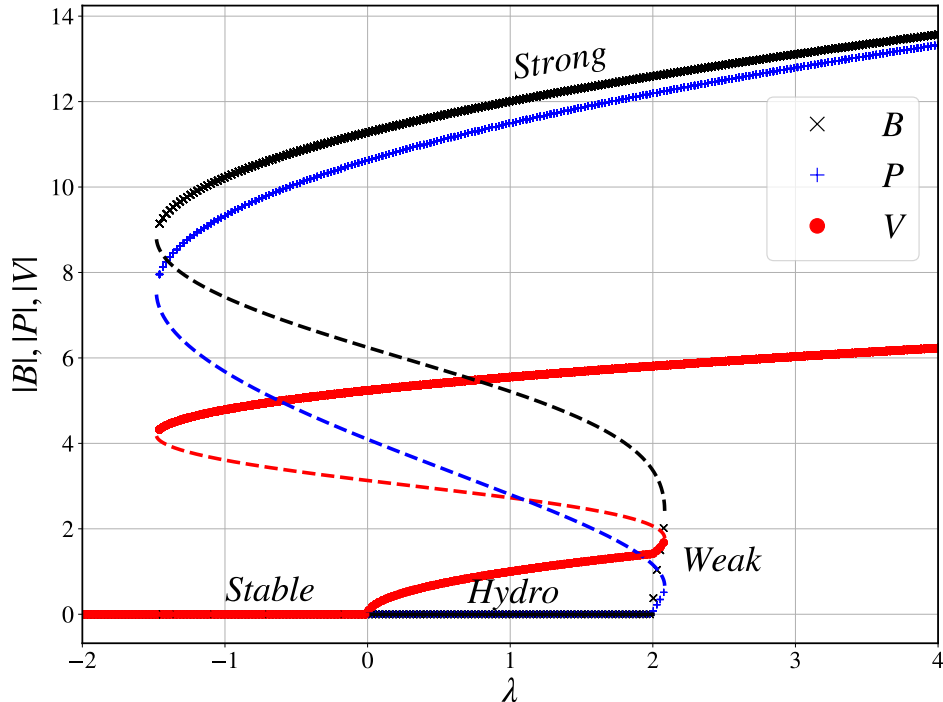
FIG. 9. Bifurcation diagram for the amplitude of each mode as \lambda varies. The parameters values are \mu = 2 , \alpha_1 = 0.2 , c_1 = 1 , \nu = 7 , \beta_1 = 0.1 , \beta_2 = 0.1 , c_2 = 1 , c_3 = 1 , \gamma = 1.2 . The points correspond to stable solutions that have been obtained by direct simulations of the system (9)-(11), while the dashed lines correspond to unstable solutions that have been computed analytically.
