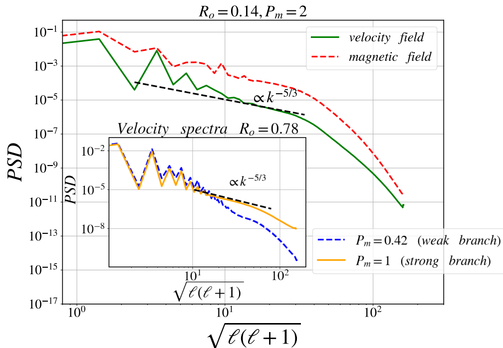
FIG. 3. Power spectrum density for the run Ro = 0.14 , Pm = 2 , Ek = 10^{-5} , N/\Omega = 1.24 , for the velocity and magnetic field, computed in the active dynamo region ( 0.4 < r/r_o < 0.6 ) and time-averaged over the saturated phase. Inset : PSD for two runs at the same Ro = 0.78 , Ek = 10^{-5} , N/\Omega = 1.24 , but for different Pm (strong and weak branches).
