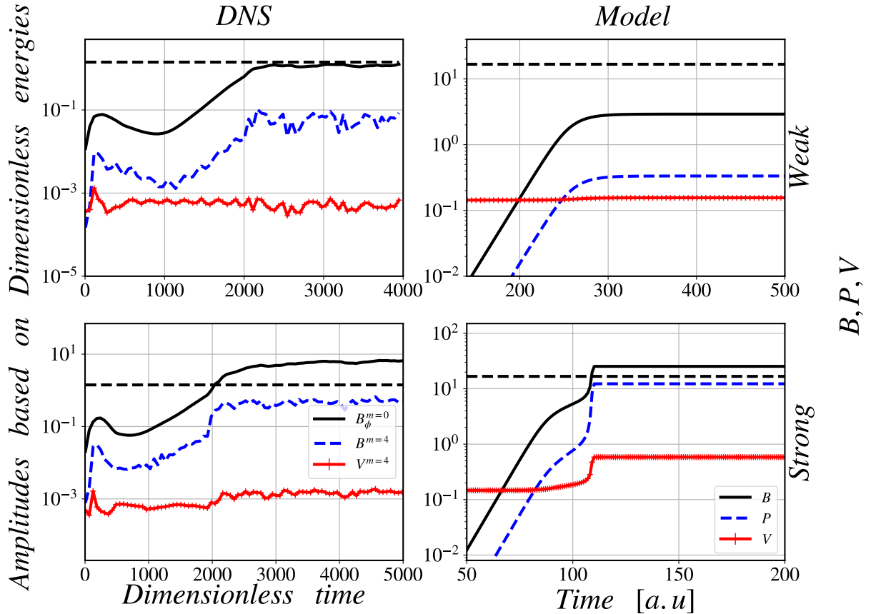
FIG. 8. Timeseries from our DNS at Ek = 10^{-5} , N/\Omega = 1.24 , Ro = 0.78 (left) compared to the ones from the model derived here (right) for the weak (top, Pm = 0.42 ) and the strong (bottom, Pm = 1 ) dynamo branches. The horizontal dashed lines correspond to Tayler instability threshold, computed locally as in [36]. For DNS, we plot \sqrt{\Lambda} for the magnetic field, and \sqrt{E_{kin}} for the velocity field, where E_{kin} is obtained by averaging the full kinetic energy on the whole volume on the saturated phase. Equations (9)-(11) of the nonlinear model are integrated using the Odeint module of Python, with \mu = 2 , \alpha_1 = 0.05 , c_1 = 100 , \nu = 7 , \beta_1 = 0.1 , \beta_2 = 0.025 , c_2 = 5 , c_3 = 100 , \gamma = 0.06 , using \lambda = 2.05 (weak) or \lambda = 2.15 (strong).
